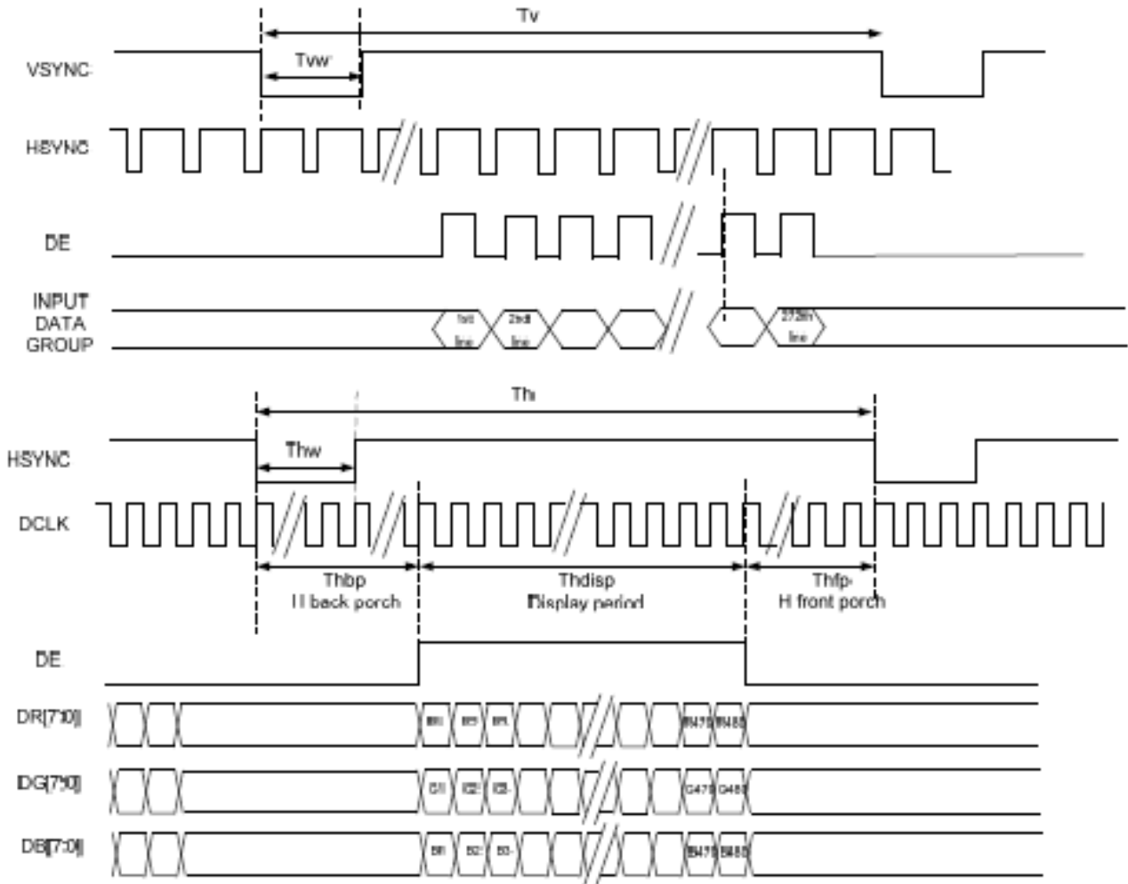
DE Mode Timing Diagram
